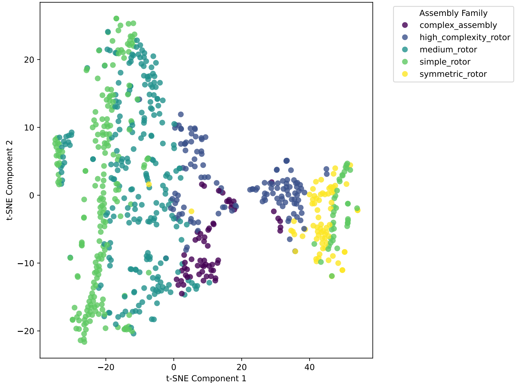
t-SNE Visualization of Engineering Assemblies
